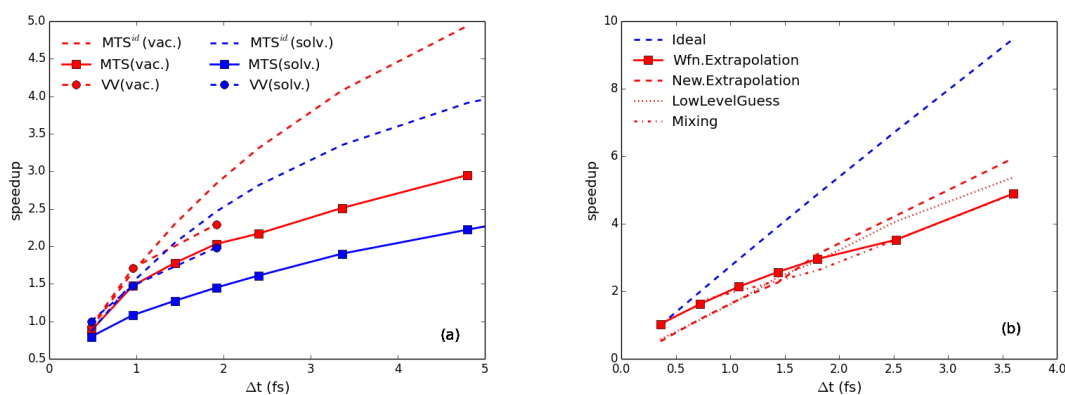
Figure 6: MTS Speedup. Panel a): acetone molecule in vacuum (red curves) and in water (blue curves); Panel b): 32 water molecules, relative to different initial guesses of the wavefunction.
