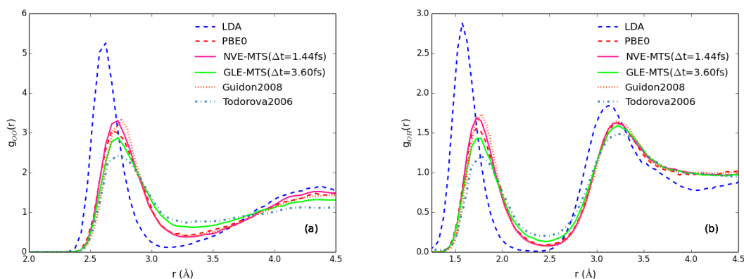
Figure 4: (a) Oxygen-oxygen and (b) intramolecular oxygen-hydrogen radial distribution functions obtained with LDA-VV MD (blue, dashed), PBE0-VV (red, dashed), LDA/PBE0 NVT-MTS MD (magenta) and GLE-MTS (green). For comparison, the same quantities from Ref. 22 (orange, dotted) and Ref. 44 (light blue, dot-dashed) are shown.
