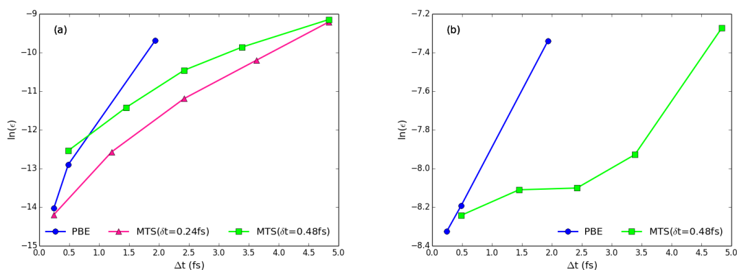
Figure 2: Logarithm of the average total energy fluctuation \varepsilon as a function of the time step of integration, over VV and MTS n NVE trajectories of 26ps for (a) an isolated acetone molecule and (b) an acetone molecule in water. All the trajectories relative to the same system were started from the same initial conditions, as described in Section 3.1. Lines are guides to the eyes.
